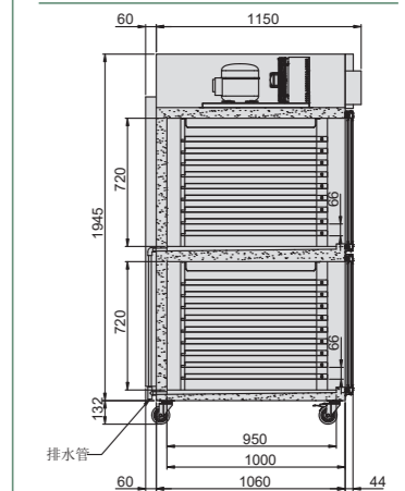
侧视图 Side View
