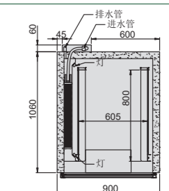
侧视图 Side View
